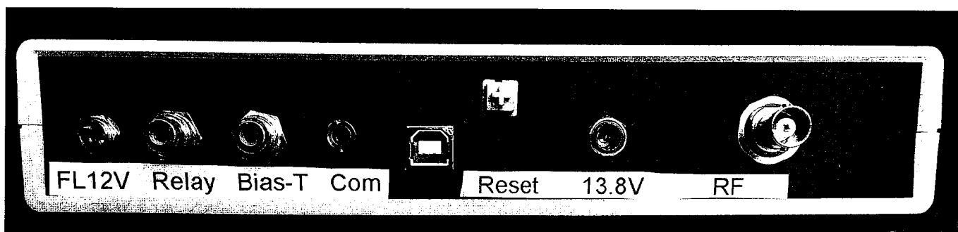
Figure 5—This photo shows the controller rear panel. The various input and output connections are shown.
