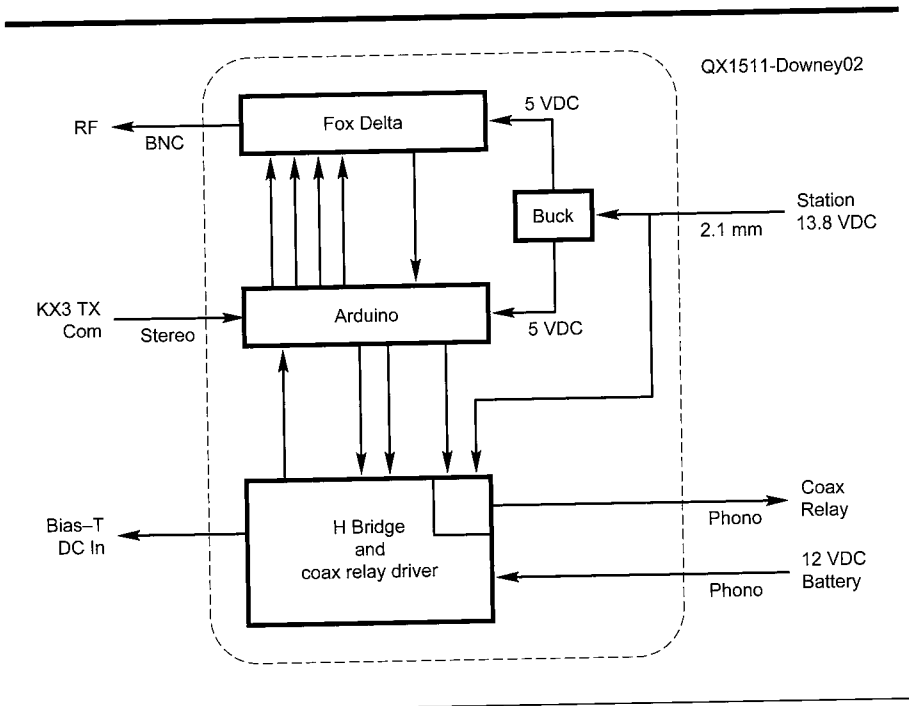
Figure 2 — This is a more detailed block diagram of the antenna tuner.
