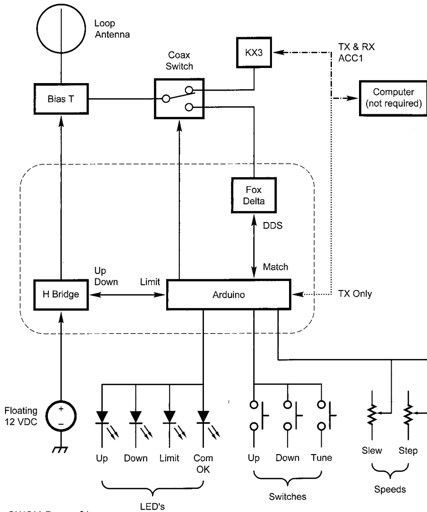
Figure 1 — This combination block diagram and simplified schematic diagram shows the basic construction of the automatic antenna controller.
