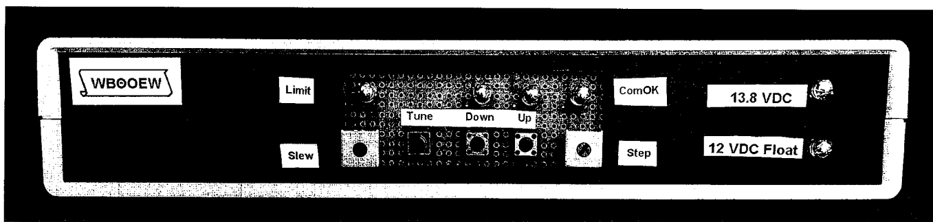
Figure 4—Here is a photo of the controller front panel. You can see the SLEW and STEP potentiometers, the TUNE, DOWN and UP pushbutton switches and the various indicator LEDs.
