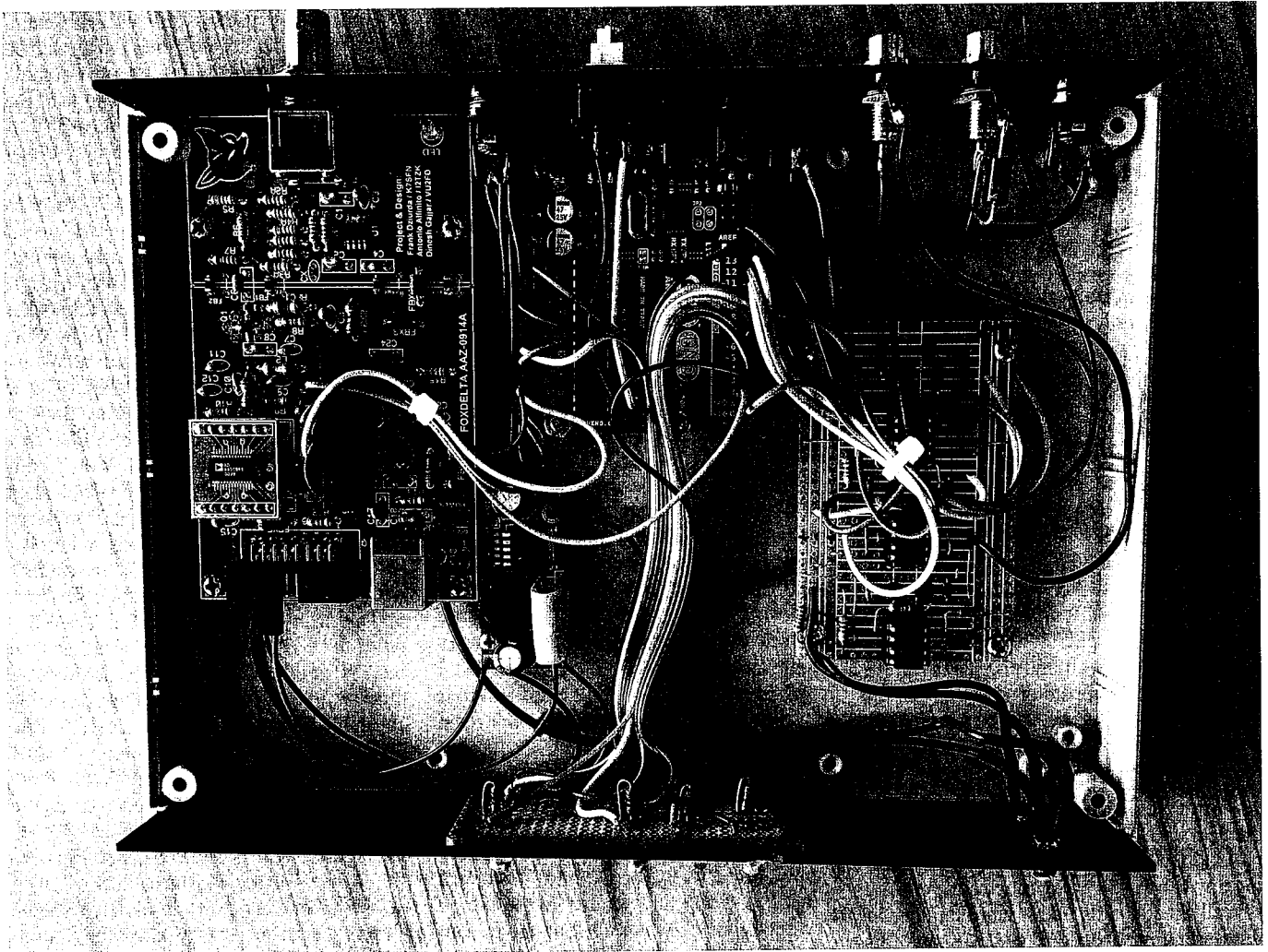
Figure 6 — Here is a photo of the wiring inside the controller cabinet. You can see the Fox Delta Antenna Analyzer boards, the Arduino board and the construction of the rest of the circuit on several perf boards.
